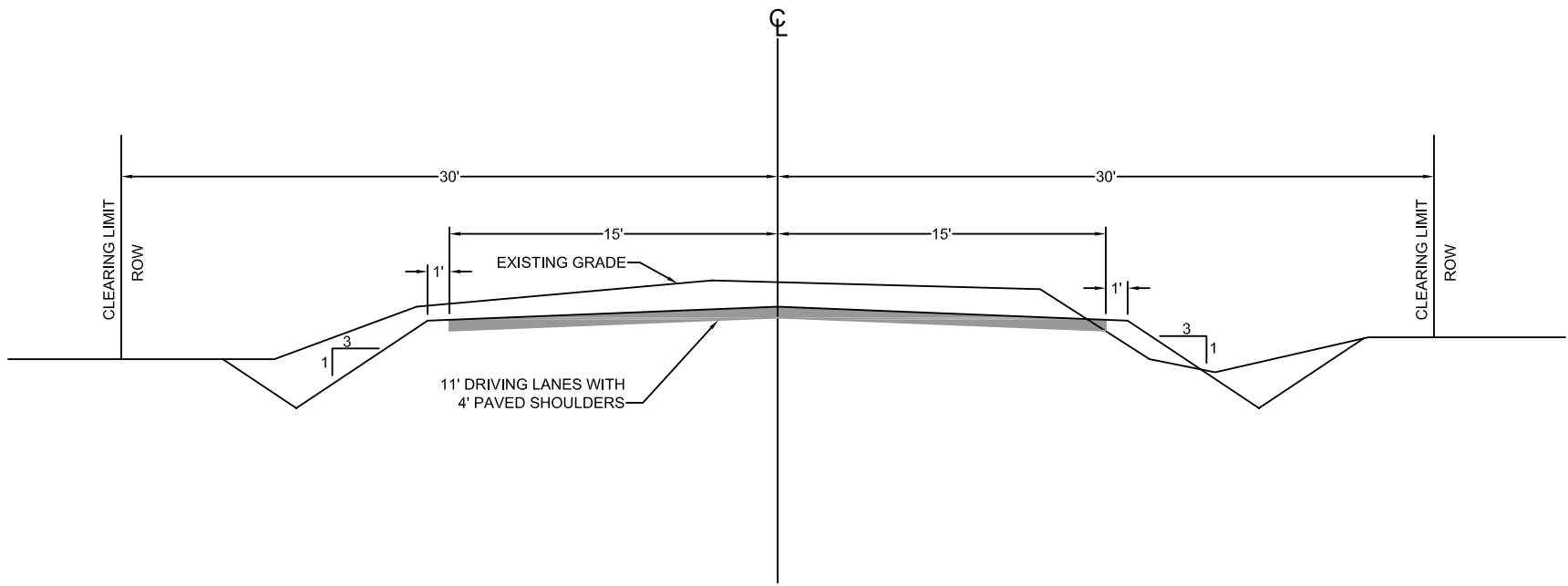
NOT TO SCALE KEYSTONE DRIVE TYPICAL SECTION
